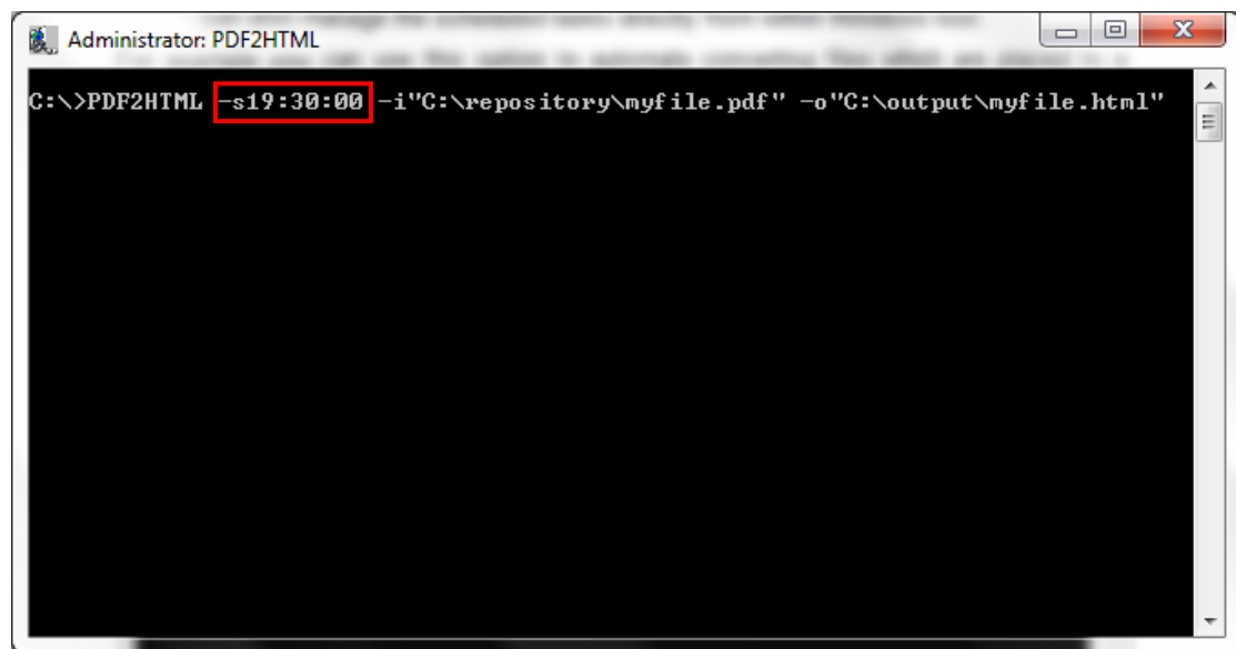
Figure 13: Scheduling the conversion (step 1/2)
