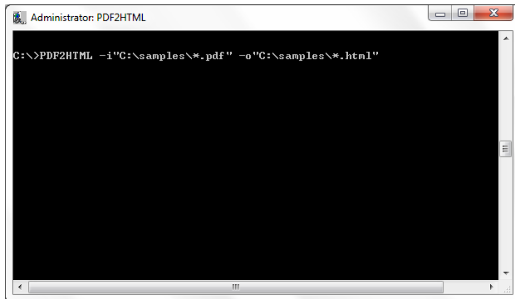
Figure 19: Converting Multiple Files Using Wildcards (step 1/2)
