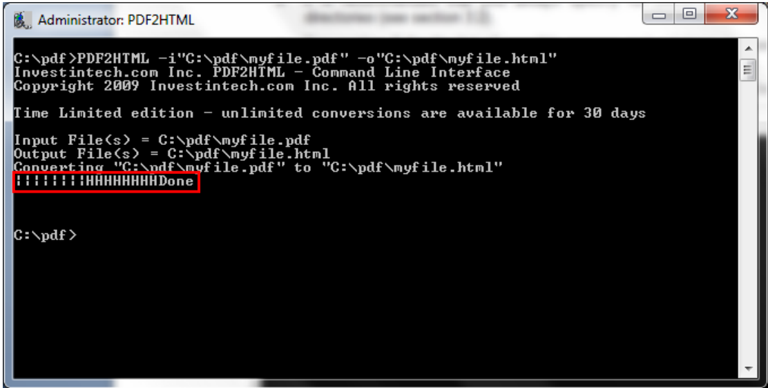
Figure 10: Conversion successful
