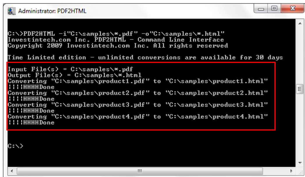
Figure 20: Converting Multiple Files Using Wildcards (step 2/2)
